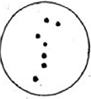
Big Dipper
