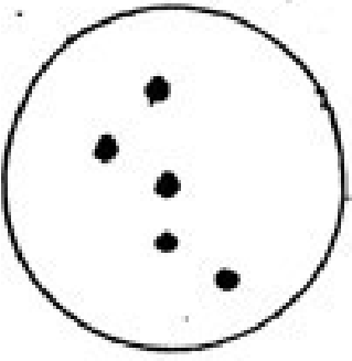
Cassiopeia
