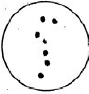
Big Dipper
