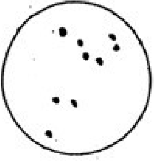
Leo
