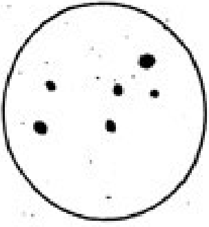
Lyra
