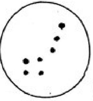
Little Dipper
