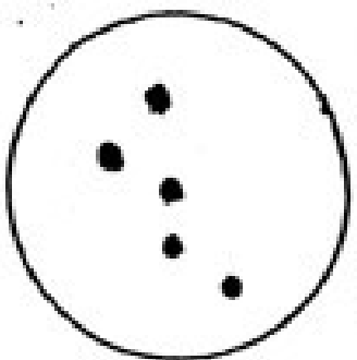
Cassiopeia
