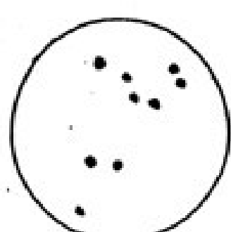
Leo
