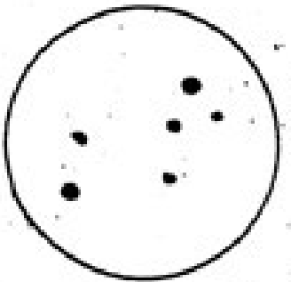
Cassiopeia
