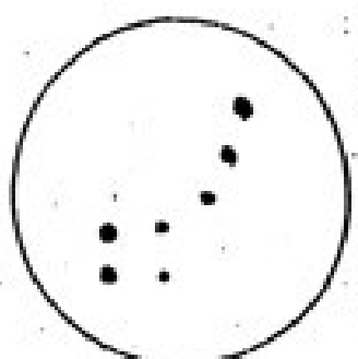
Little Dipper
