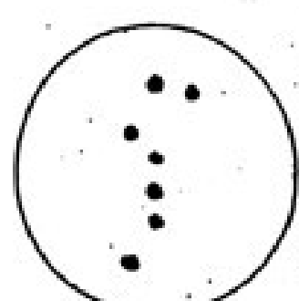
Big Dipper
